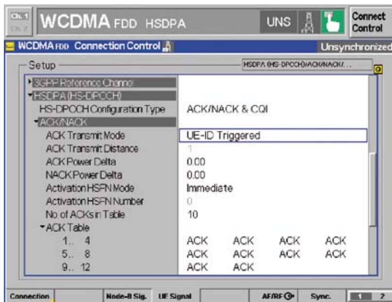
HSDPA uplink generator configuration.
